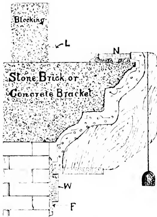
NO. 44.—PLUMBING RUNNING MOLDS.
